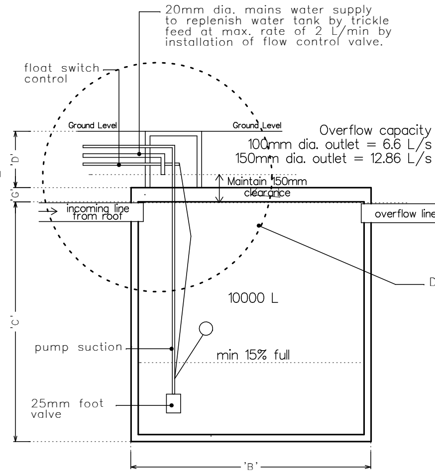
water re-use tank details scale 1:20
