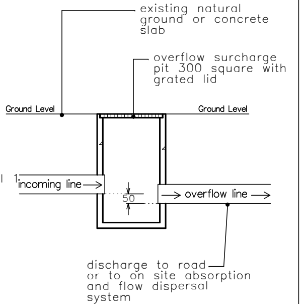
surcharge pit scale 1:20
