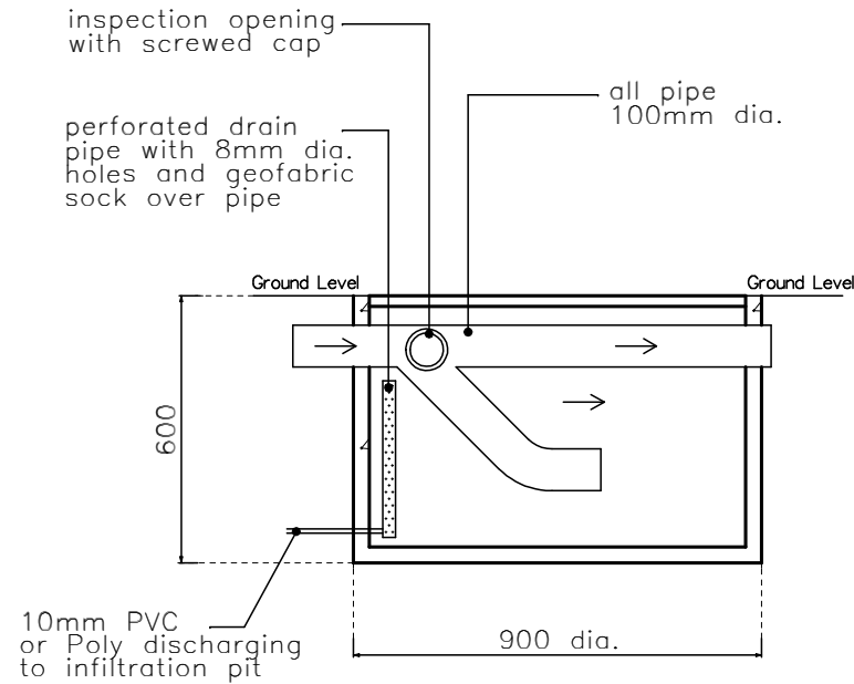
first flush system scale 1:20
