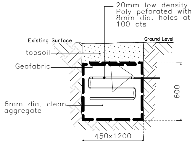
infiltration pit scale 1:20
